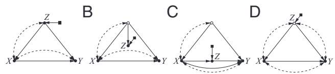
Fig. 5. Selection diagrams depicting differences between source and target populations. In A , the two populations differ in age ( Z ) distributions (so S points to Z ). In B , the populations differ in how reading skills ( Z ) depend on age (an unmeasured variable, represented by the open circle) and the age distributions are the same. In C , the populations differ in how Z depends on X . In D , the unmeasured confounder (bidirected arrow) between Z and Y precludes transportability.
