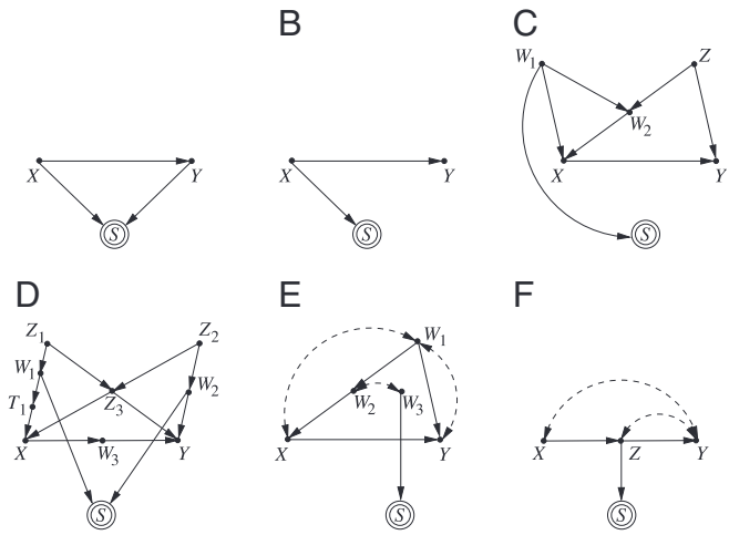
Fig. 4. Canonical models where selection is treatment dependent in A and B and also outcome dependent in A. More complex models in which W_1, W_2 and Z are sufficient for adjustment, but only the latter is adequate for recovering from selection bias, are shown in C. There is no sufficient set for adjustment without external data in D F. (D) Example of S -backdoor admissible set. (E and F) Structures with no S -admissible sets that require more involved recoverability strategies involving posttreatment variables.
