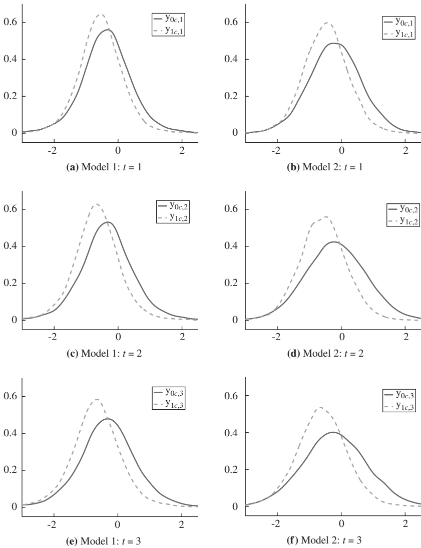
Fig. 4. Predictive Marginal Distributions of the Potential Outcomes for Compliers in Models 1 and 2.
