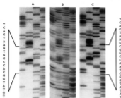
Fig. 2. Evidence for multiple alleles in the 18S rDNA sequence(s) obtained from A. parviflora GEda. B , Overlapping sequence obtained directly from the PCR products using primer 892a (11, 32). A , C , Two different sequences obtained after cloning the PCR products. The sequences are located in sters 29.1 approximately at base 1321 in GEda. The sequence reads in the 5' to 3' direction from the bottom to the top. The two sequences indicate the presence of two different alleles.
