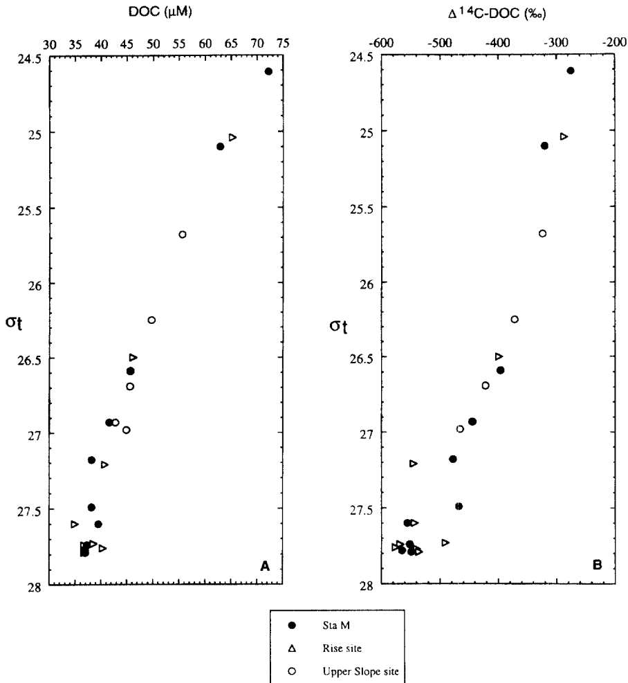
Fig. 7. DOC concentrations and \Delta^{14}\text{C-DOC} values at the three study sites plotted as a function of temperature-corrected density ( \sigma_t ). (A) Concentrations for the full range of \sigma_t over all depths measured; (B) \Delta^{14}\text{C-DOC} values for the full range of \sigma_t over all depths measured.
